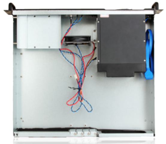
Inside view
